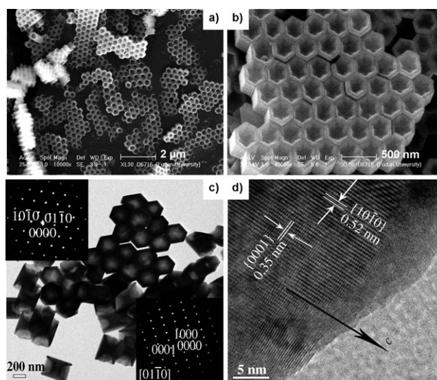
Figure 1. a), b) SEM images of arrays of hexagonal nanotubes of \beta\text{-NaYF}_4 . c) TEM image of the nanotubes and corresponding ED patterns (insets). d) HRTEM image of a nanotube.
